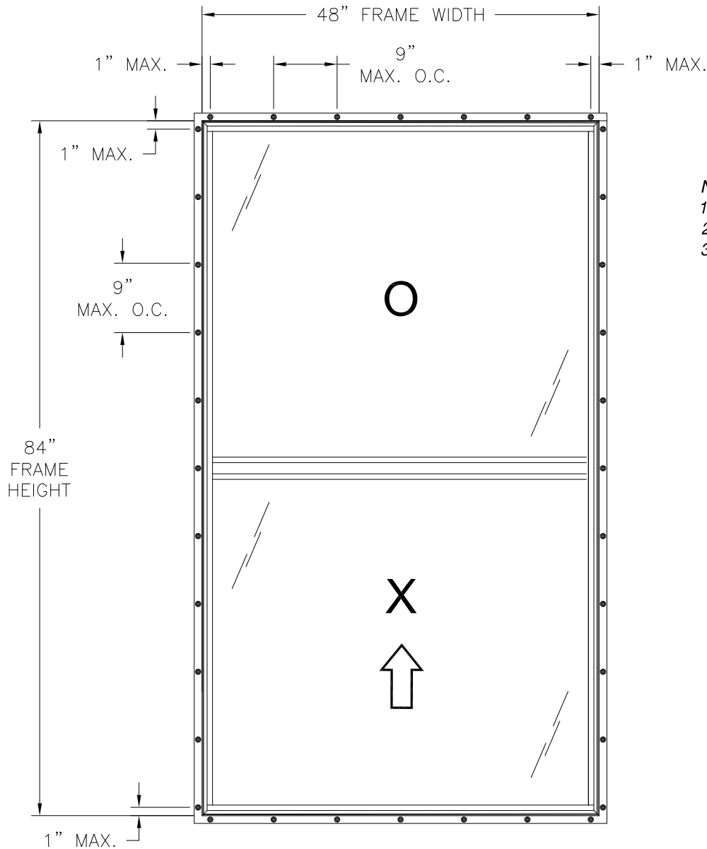
400/475 VINYL SINGLE HUNG TILT WINDOW EXTERIOR VIEW
