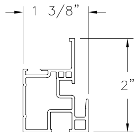
MEETING RAIL (4004) EXTRUDED RIGID PVC
