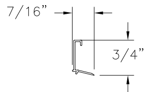
GLAZING BEAD (DT1720-R) EXTRUDED RIGID PVC
